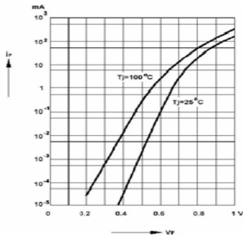
Forward characteristics
