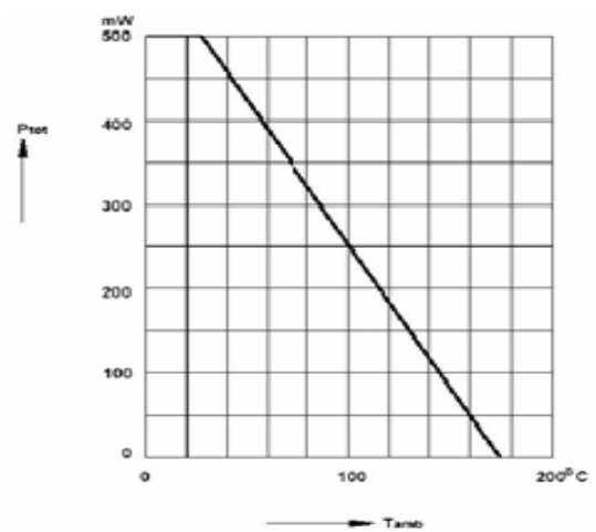
Admissible power dissipation versus ambient temperature
