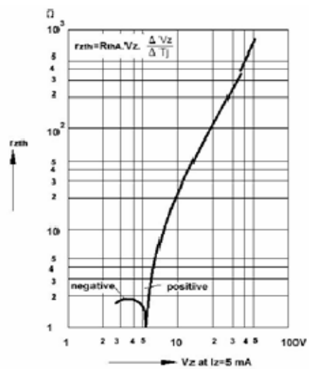
Thermal differential resistance versus Zener voltage
