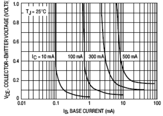
Figure 2. Saturation Region
