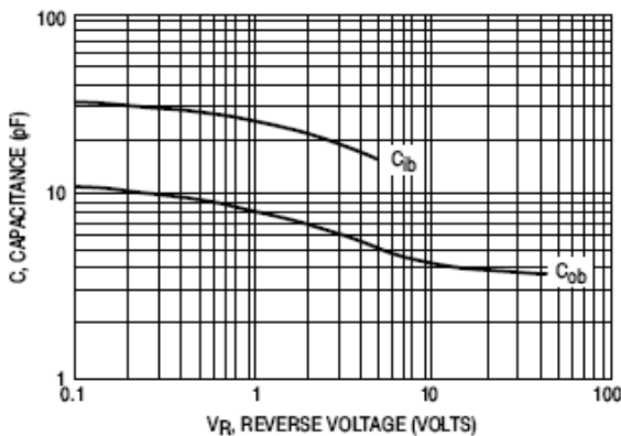
Figure 5. Capacitances
