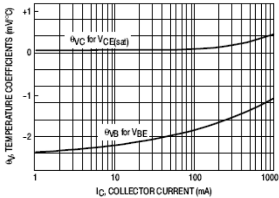
Figure 4. Temperature Coefficients
