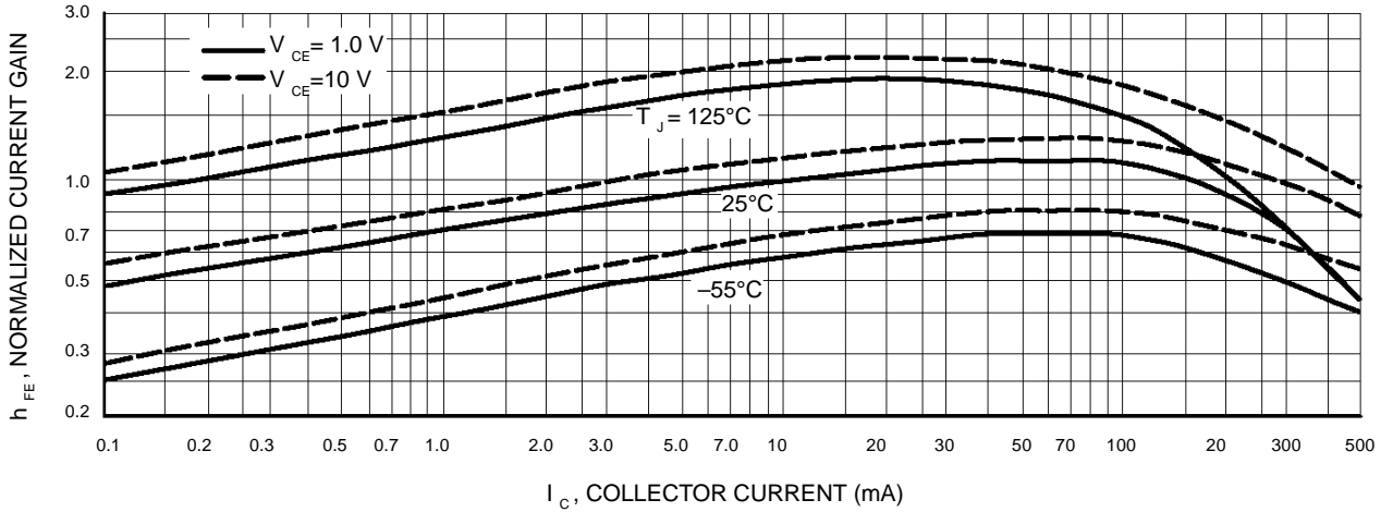
Figure 11. DC Current Gain
