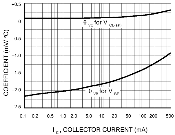
Figure 14. Temperature Coefficients
