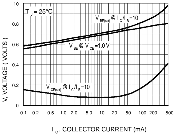
Figure 13. "On" Voltages
