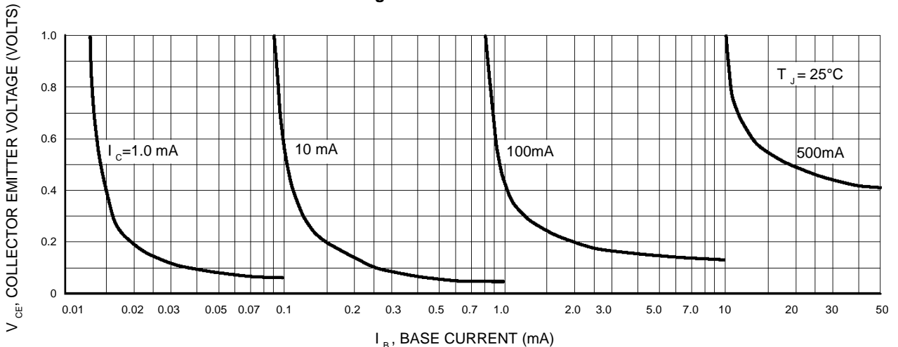
Figure 12. Collector Saturation Region
