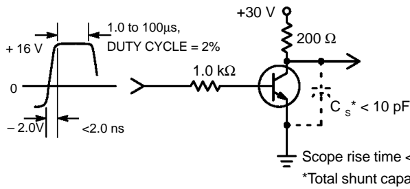
Figure 1. Turn-On Time
