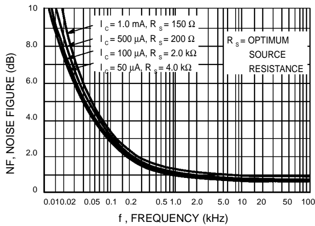
Figure 3. Frequency Effects
