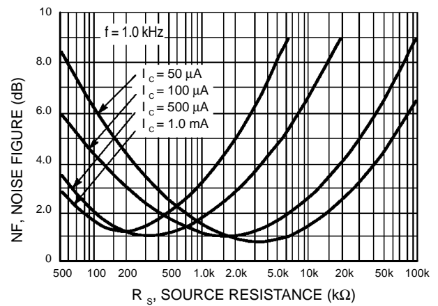
Figure 4. Source Resistance Effects
