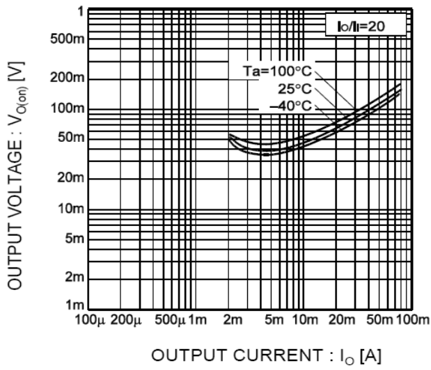
Fig.5 Output voltage vs. output current
