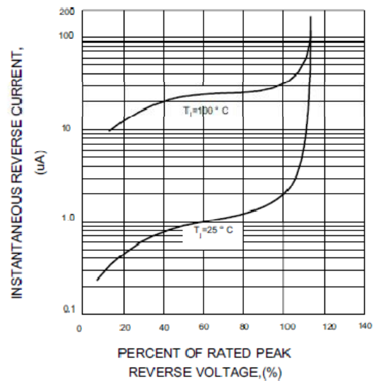
FIG.4-TYPICAL REVERSE CHARACTERISTICS
