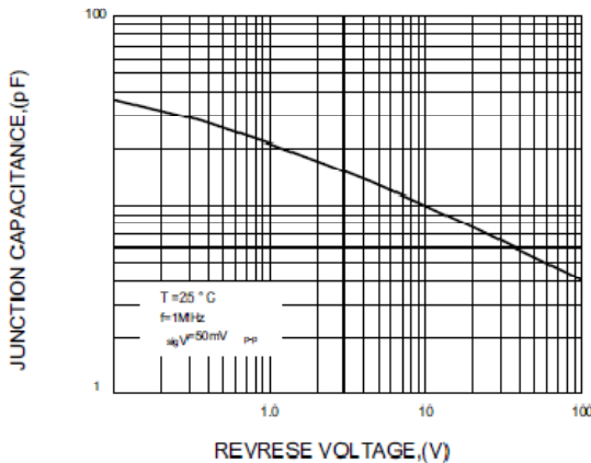
FIG.5-TYPICAL JUNCTION CAPACITANCE
